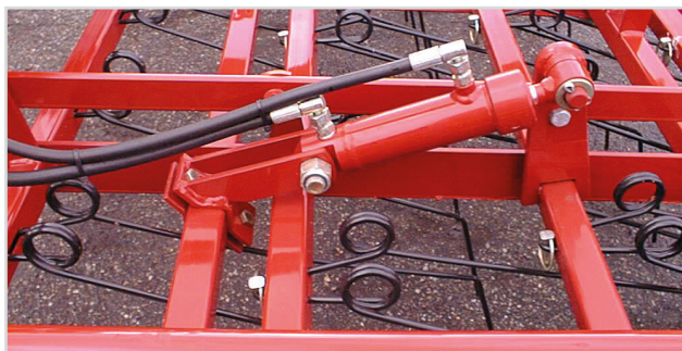
Hydraulically adjustable tine pressure.
